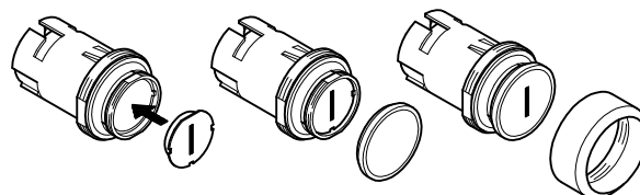
Insert assembly
