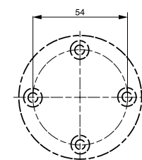
Drilling plan for signal towers K 70
